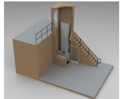
Straight Through Shaftway Application Shown
